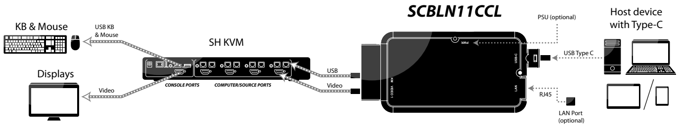
USB Type-C to DP SH KVM Cable System Diagram
