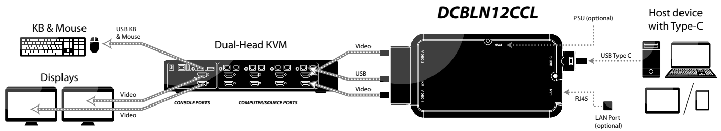
USB Type-C to DP Dual-Head KVM Cable System Diagram
