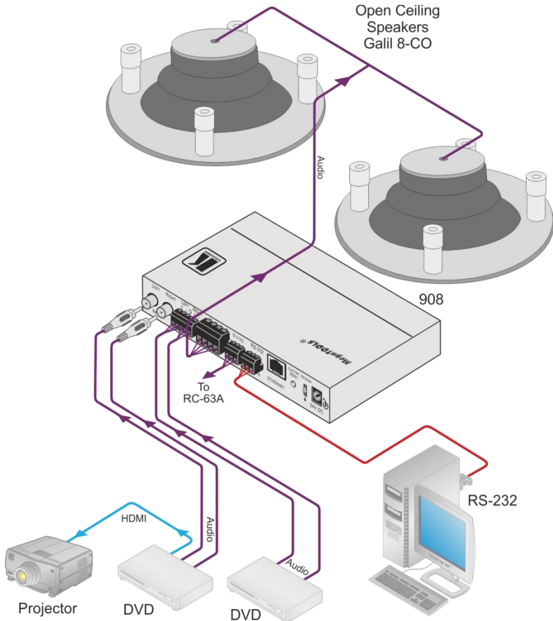
Figure 1: Open-back Ceiling Speakers in a Boardroom Setup
