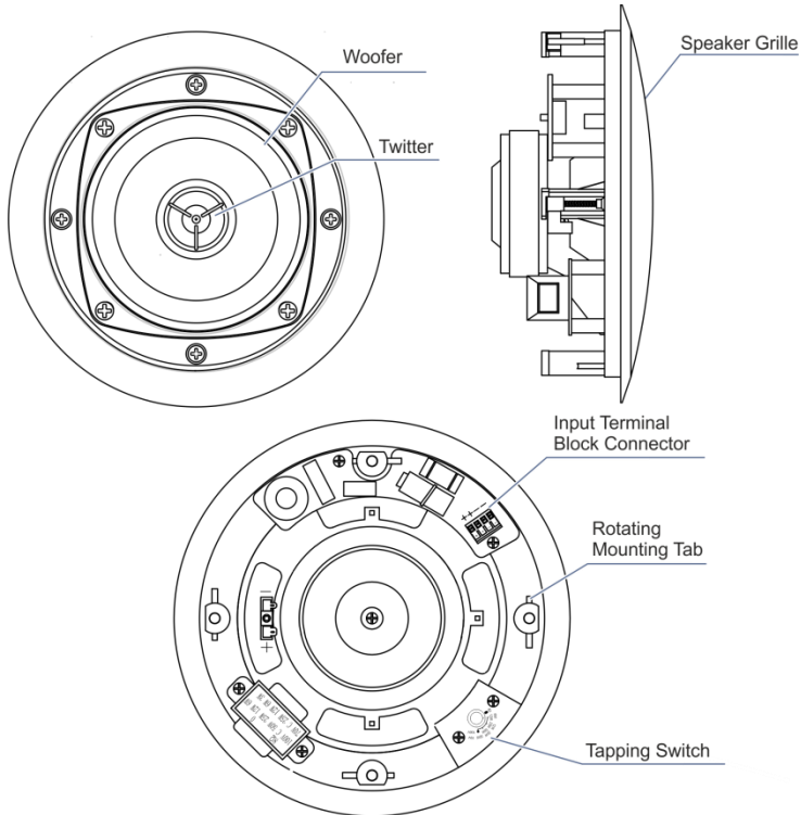
Figure 2: Galil 8-CO Open-back Ceiling Speakers
